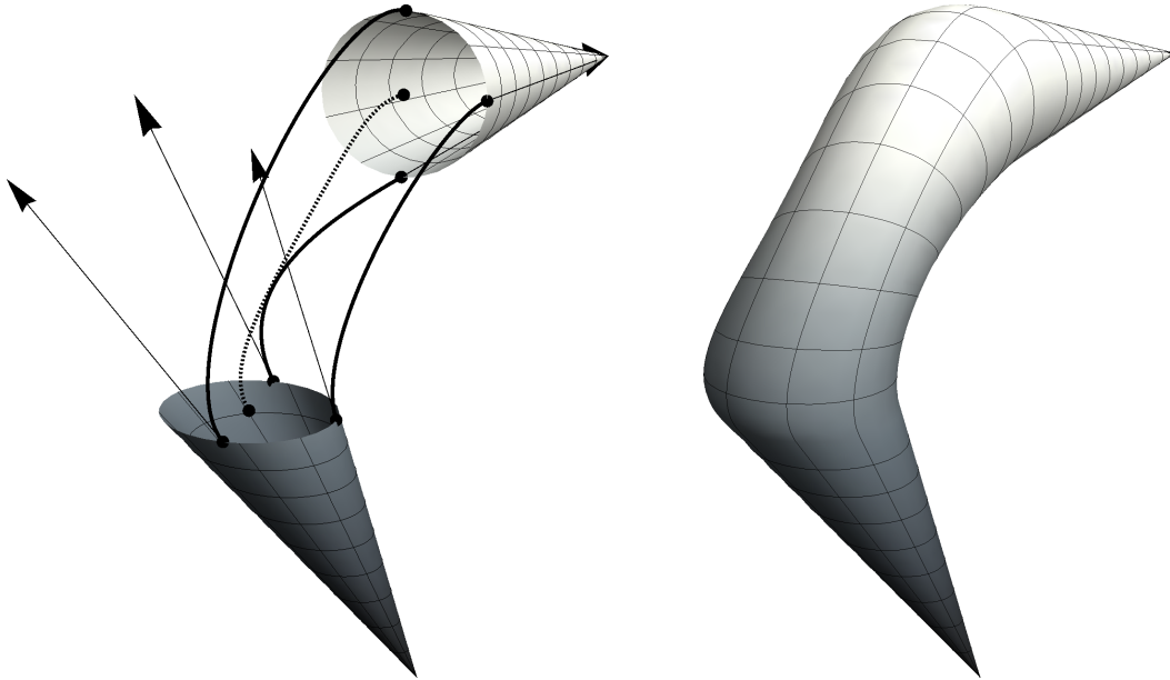
Figure 6: Left: Two given ringed surfaces (quadratic cones), three cubic curves interpolating sampled data (solid) and the computed directrix curve (dashed); Right: The final blending ringed surface.
