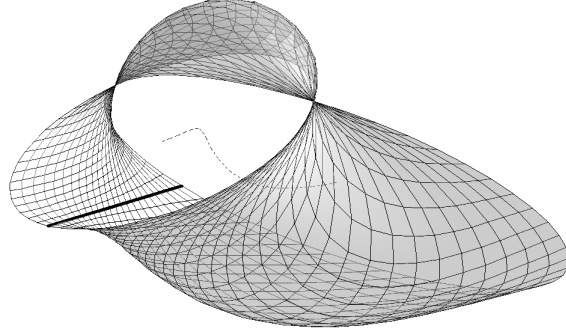
Figure 2: Applying PRRS to a line and two points (Example 3): The given line \ell_1(u) (solid), the directrix \mathbf{c}(u) (dashed) and the obtained ringed surface \mathbf{x}(u, v) for u \in [-2, 2] from Example 3. The two singularities are exactly the points \mathbf{P}_2 and \mathbf{P}_3 .
