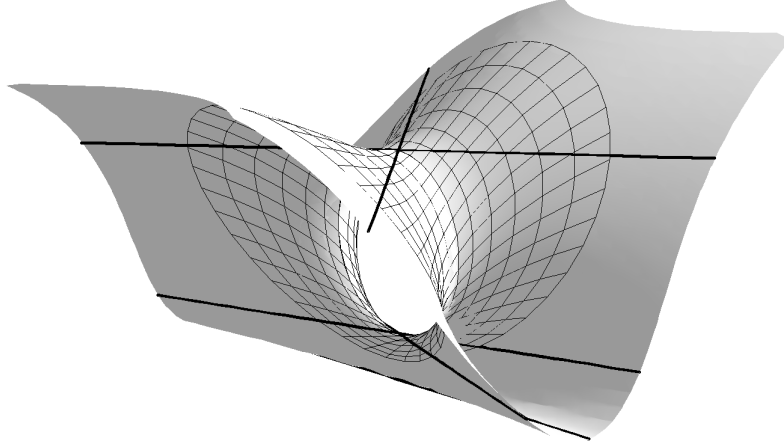
Figure 4: The algebraic surface C from Example 2 (continued) and the five real lines on it.
