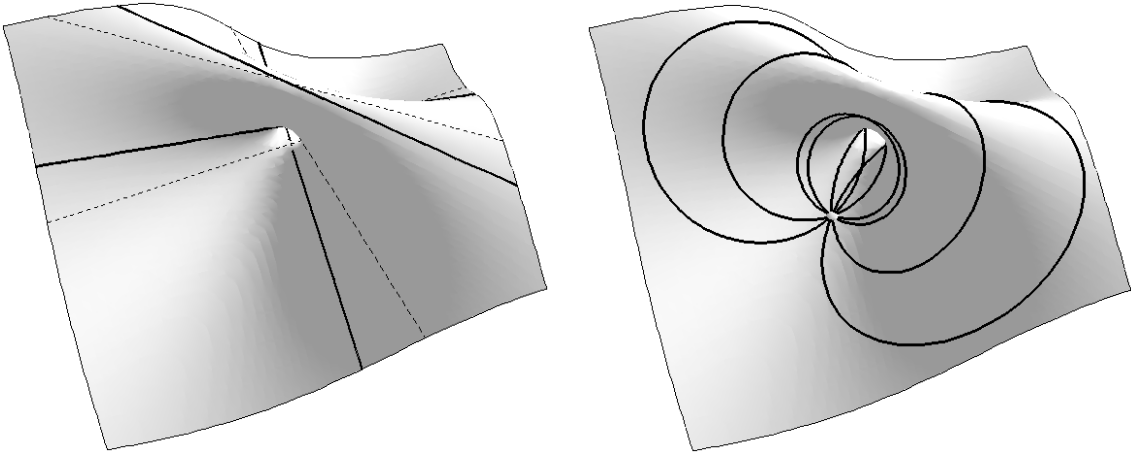
Figure 3: The parabolic Darboux cyclide C for \alpha = 0 from Example 4. Left: The three given lines \ell_i ( i = 1, 2, 3 ) (solid) and the additional three lines \widehat{\ell}_i (dashed). Right: Six circles on the surface through the point (2, -2, -1)^\top .
