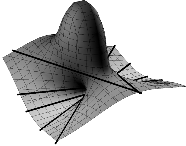
Figure 5: The parabolic Darboux cyclide C from Example 5 with six real lines on it.
