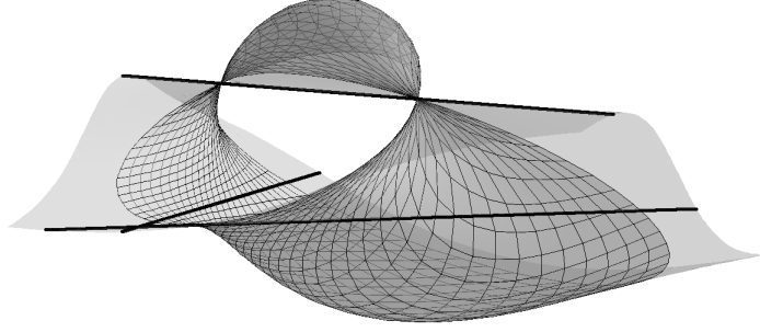
Figure 7: The algebraic surface C from Example 3 (continued) and the three real lines on it.
